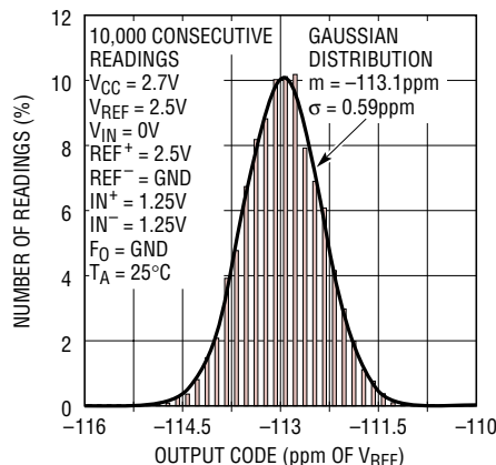
Long-Term Histogram (60Hrs)
