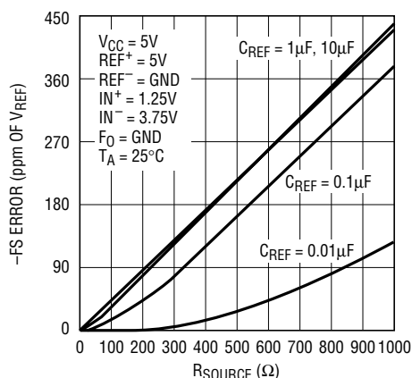
Figure 28. -FS Error vs R_{SOURCE} at REF^+ and REF^- (Large C_{REF} ) sn2415 24151fs
