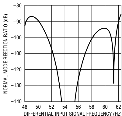
Figure 33. Normal Mode Rejection when Using an Internal Oscillator
