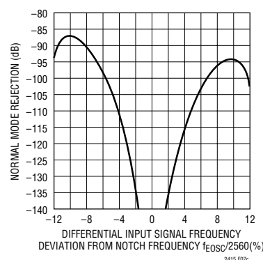
Figure 7c. LTC2415/LTC2415-1 Normal Mode Rejection When Using an External Oscillator of Frequency f_{EOSC} with Running Averages
